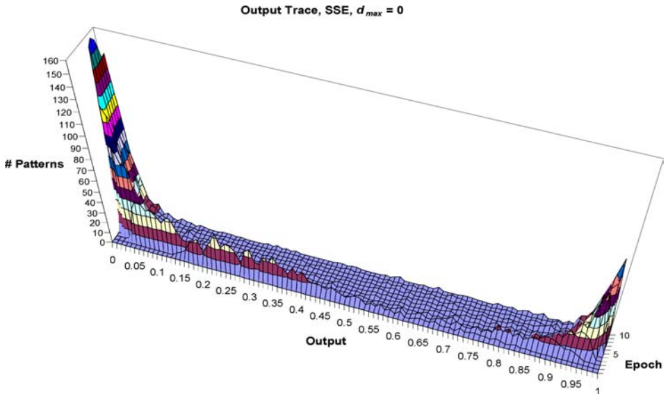
Fig. 4 Network output trace SSE optimization on bcw (first ten epochs). Weight saturation occurs after only a few training epochs
