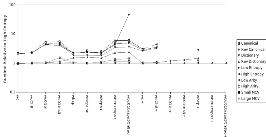
Fig. 17. Runtime in minutes of each ordering strategy relative to High Entropy feature ordering (lower is better). A value of 10 is 10 times worse than High Entropy. Again, the orderings tend towards two main groups (although Dictionary and Reverse Dictionary again show some deviation from this.)
