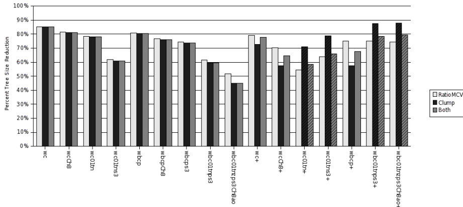
Fig. 5. Percent tree size reduction relative to the baseline (higher is better). Bars with hash marks did not finish constructing the tree due to memory complications.
