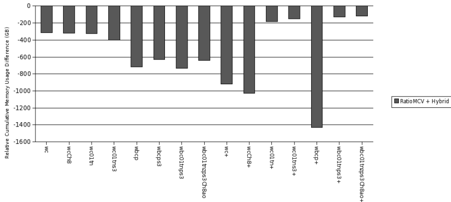
Fig. 15. Difference in cumulative memory usage (in GB) relative to the RatioMCV results in Figure 14 (lower is better). Again, the bars with hash marks presumably would have continued the trends if all queries had been completed.
