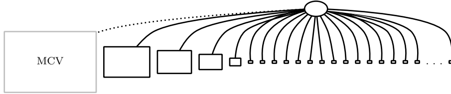
Fig. 2. Vary node for a feature with skewed MCV (high proportional count). Relative node size represents the relative counts at each node (as well as the a priori potential size of the corresponding subtrees). Although it is still necessary to sum over many nodes to recover some queries, the MCV subtree is so large and the potential for further MCV collisions in the smaller subtrees so small that the trade-off is more reasonable (contrast Figure 1).
