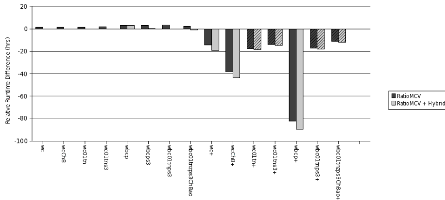
Fig. 12. Relative difference in runtime (in hours) from the baseline (lower is better). The improvement in runtime is not always large but it is consistent across (almost) all feature sets. It also consistently larger for larger feature sets since the partial static amortizes a larger percentage of the work done constructing the tree. Bars with hash marks did not finish all of the queries in the respective query logs due to memory complications.
