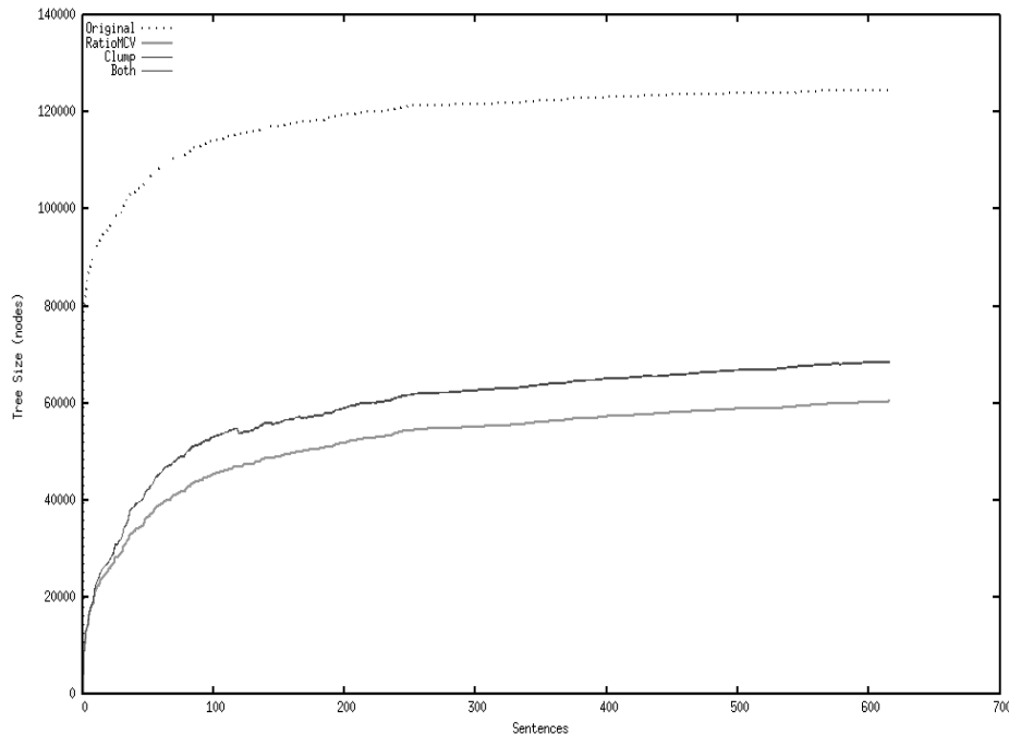
Fig. 8. Example of how tree size varies as sentences are tagged using the feature set wbc01tnzps3Ch8ao . Tree growth tapers off towards the right as fewer unique words (and correspondingly unique value assignments) are encountered. Although using a clump node does slightly increase tree size, it is still significantly less than the unmodified tree.
