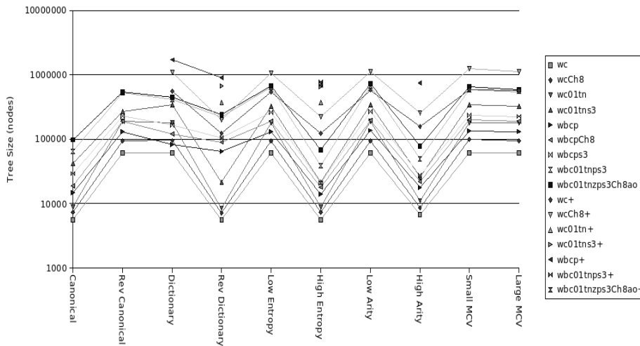
Fig. 18. Actual tree size of each ordering strategy (lower is better). The x -axis is sorted such that pairs of forward and reverse ordering strategies are next to each other. Note the log scale for the y -axis. Most of the pairs have one ordering which clearly outperforms the other. Only the orderings related to MCV both perform poorly.
