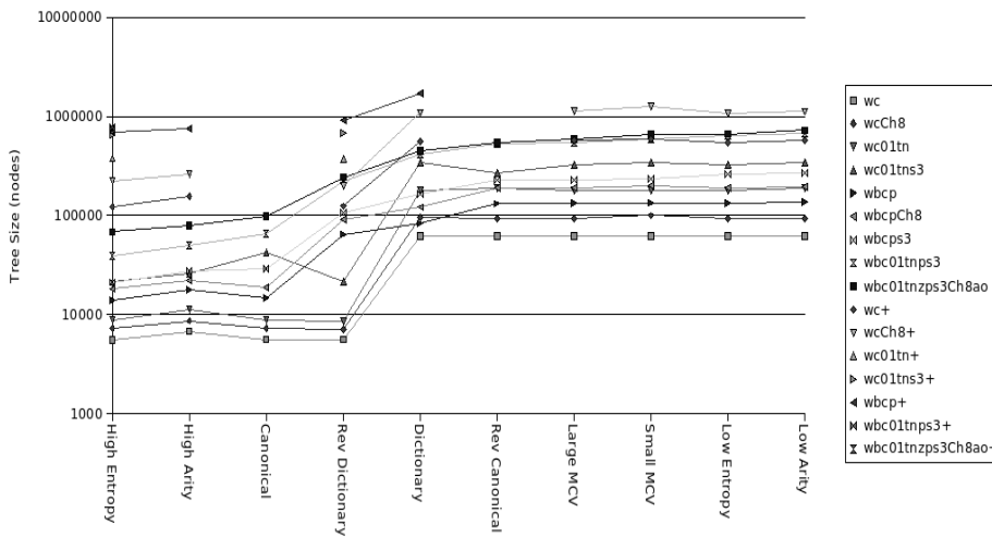
Fig. 19. Actual tree size of each ordering strategy (lower is better). The x -axis is sorted according to the tree size obtained by wbc01tnzps3ch8ao . This sorting more clearly illustrates the two basic groups of orderings. Note the log scale for the y -axis.
