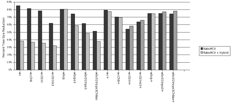
Fig. 10. Percent tree size reduction relative to the baseline (higher is better). Because the same partial static tree is used for each feature set, the smaller feature sets actually perform much worse. Bars with hash marks did not finish all of the queries in the respective query logs due to memory complications.
