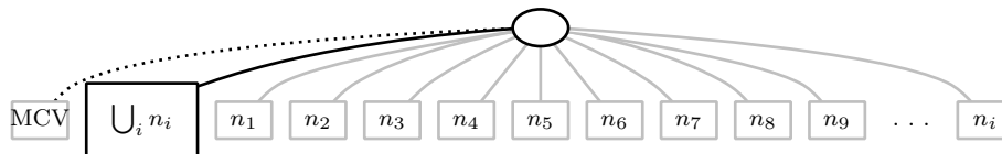
Fig. 3. Here the issue of skew is ignored and so the nodes are represented as uniform in size. However, the Clump node represents both the sum of the counts of the other nodes as well as the union of the rows (represented here) for that node’s partition of the dataset.
