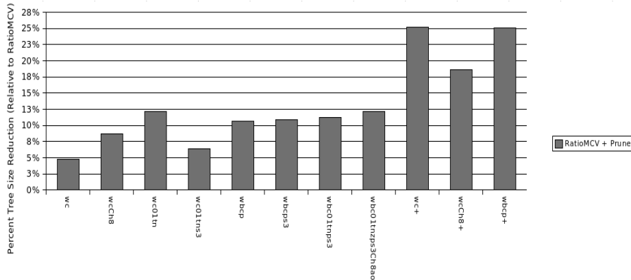
Fig. 24. Percent tree size reduction relative to the RatioMCV results in Figure 23 (higher is better). Here the trend of improved performance as feature set size increases is fairly clear.
