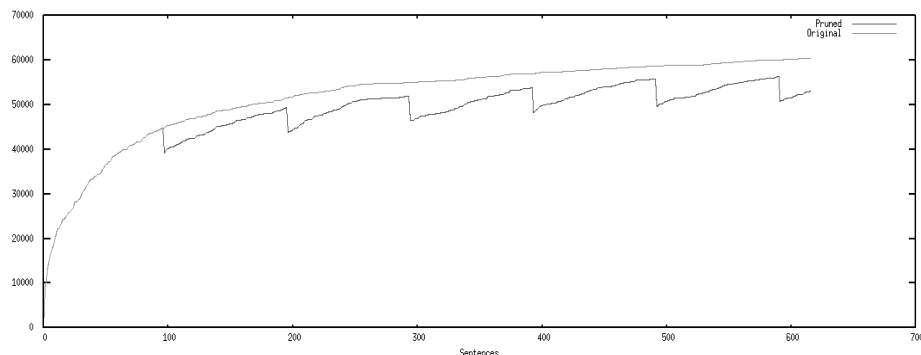
Fig. 22. Example of how tree size varies as sentences are tagged using the feature set wbc01tnzps3Ch8ao with and without pruning. The pruning strategy only removes a small percentage of the tree, some of which is re-built over the course of subsequent queries.
