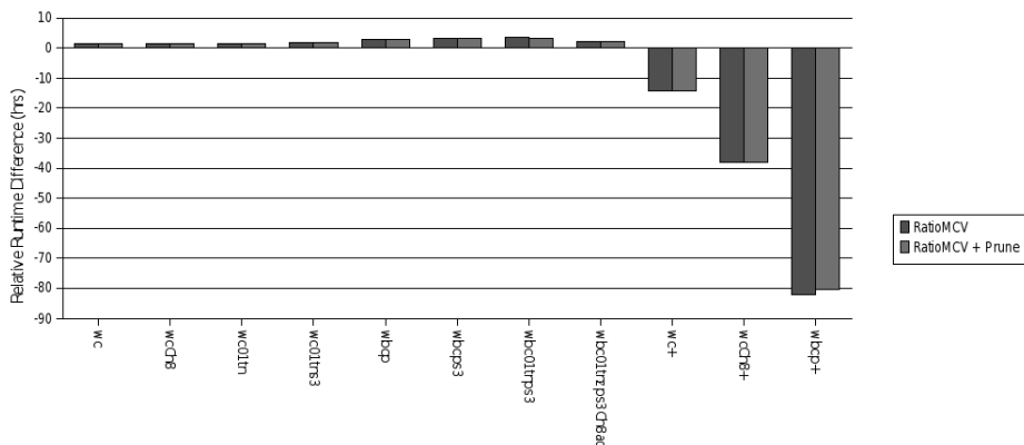
Fig. 25. Relative difference in runtime (in hours) from the baseline (lower is better). Pruning is a fairly inexpensive operation timewise and so the results are not significantly different.
