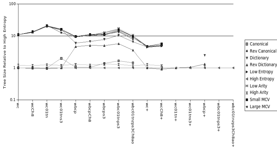
Fig. 16. Tree size of each ordering strategy relative to High Entropy feature ordering (lower is better). A value of 10 is 10 times worse than High Entropy. The ordering strategies tend to cluster into two groups, with the notable exception of Reverse Dictionary and to a lesser extent Dictionary (over only a portion of the feature sets).
