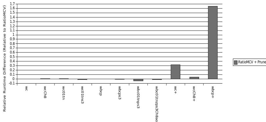
Fig. 26. Relative difference in runtime (in hours) relative to the RatioMCV results in Figure 25 (lower is better).
