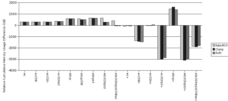
Fig. 7. Difference in cumulative memory usage (in GB) from the baseline (lower is better). Bars with hash marks did not finish constructing the tree due to memory complications.
