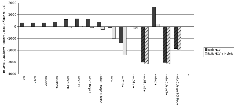
Fig. 14. Difference in cumulative memory usage (in GB) from the baseline (lower is better). Bars with hash marks did not finish all of the queries in the respective query logs due to memory complications.
