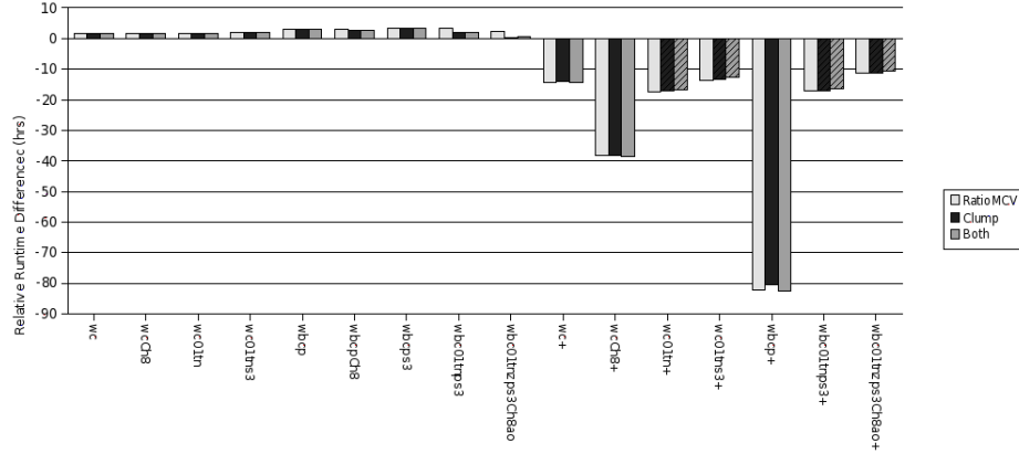
Fig. 6. Relative difference in runtime (in hours) from the baseline (lower is better). Bars with hash marks did not finish constructing the tree due to memory complications.
