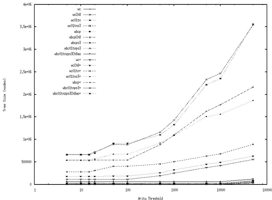
Fig. 4. Results of varying the arity threshold from 5 to 50000 on tree size (number of nodes) for each of the 16 feature sets. Notice the x -axis uses a logarithmic scale. The individual lines are less important than the overall trend. The large scale of the y -axis disguises the fact that most of the feature sets show a small upward curve at the low end of the x -axis.
