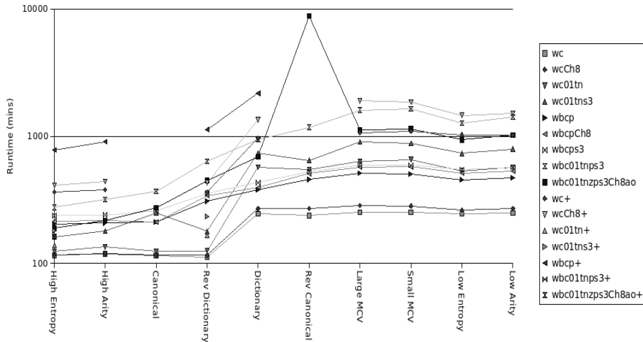
Fig. 21. Actual runtime of each ordering strategy (lower is better). The groupings remain approximately the same as with the tree size. The x -axis is sorted the same as in Figure 19. Note the log scale for the y -axis.
