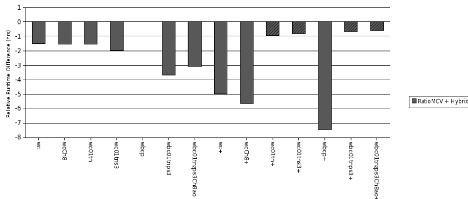
Fig. 13. Relative difference in runtime (in hours) relative to the RatioMCV results in Figure 12 (lower is better). The apparently poorer performance of those bars marked with hash marks is due to early termination caused by memory management bugs. It is reasonable to infer that the trend of increased improvement for larger feature sets would have continued without these complications.
