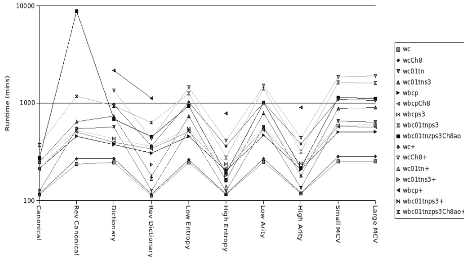
Fig. 20. Actual runtime of each ordering strategy (lower is better). The x -axis is sorted such that pairs of forward and reverse ordering strategies are next to each other. The alternating pattern of ordering pairs repeats as with tree size. Note the log scale for the y -axis.
