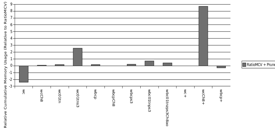
Fig. 28. Difference in cumulative memory usage (in GB) relative to the RatioMCV results in Figure 27 (lower is better).
