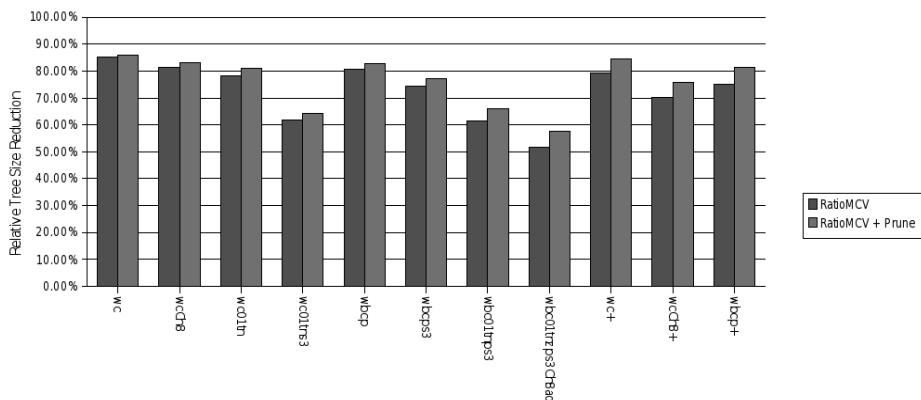
Fig. 23. Percent tree size reduction relative to the baseline when using pruning compared the results for Complete Vary Nodes and RatioMCVs (higher is better). Tree size is slightly better for all feature sets and performs the best for larger feature sets.
