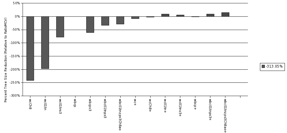
Fig. 11. Percent tree size reduction relative to the RatioMCV results in Figure 10 (higher is better). Here the poorer performance (larger tree size) for smaller feature sets is very clear. Note that since this graph does not use the baseline as a comparison point, the scale of this graph is not relevant to that of Figure 10.
