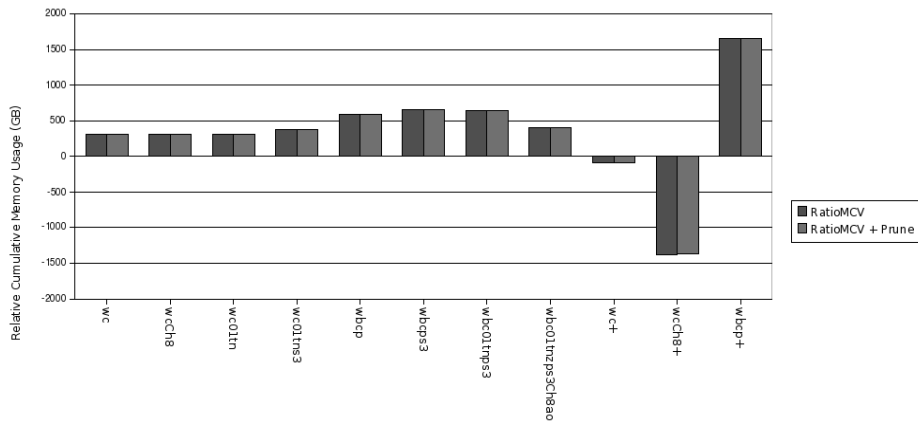
Fig. 27. Difference in cumulative memory usage (in GB) from the baseline (lower is better).
