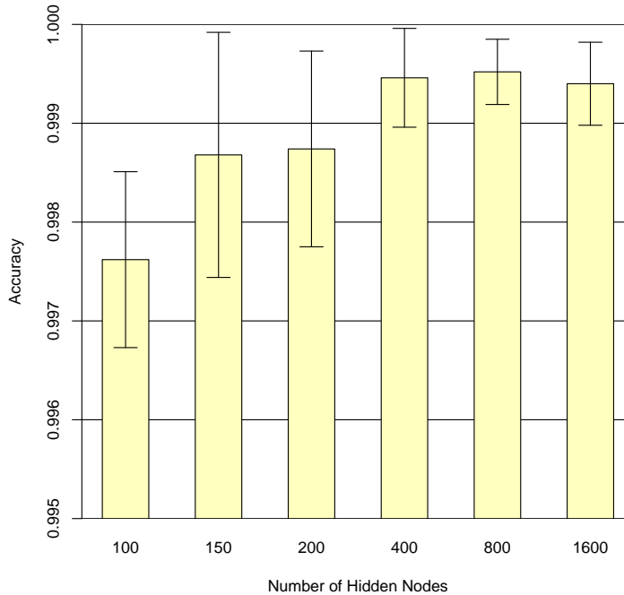
Figure 2: Mean accuracy and two standard deviations for 100 – 1600 hidden node ANNs on the 4,000-utterance ASR training set.
