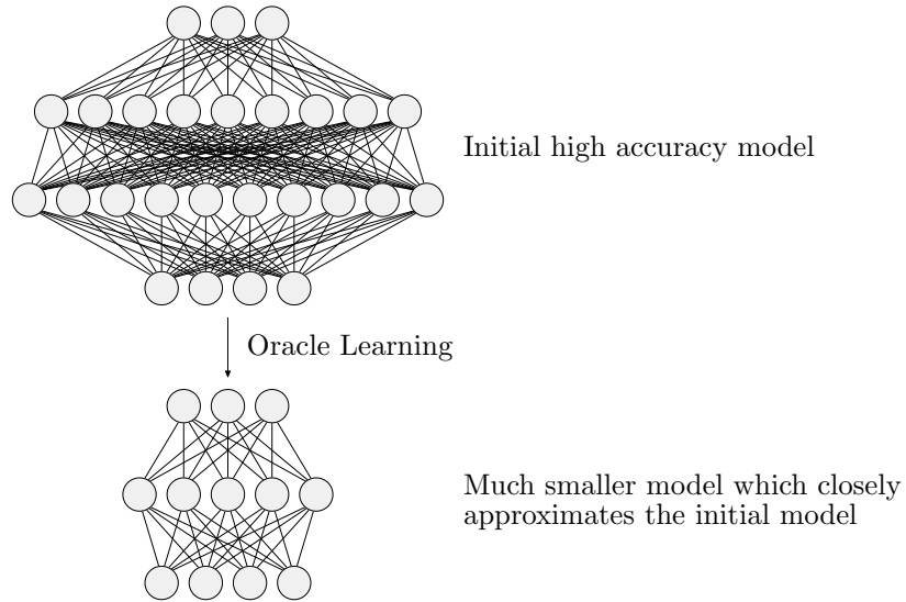
Figure 1: Using oracle learning to reduce the size of an ANN.
