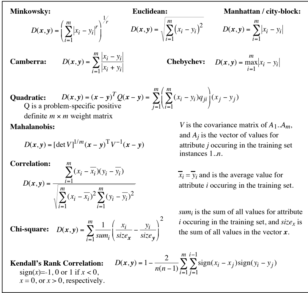
Figure 1. Equations of selected distance functions. (x and y are vectors of m attribute values).
